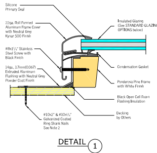
HORIZONTAL CROSS SECTION
