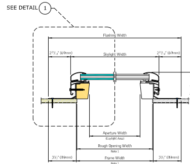
HORIZONTAL CROSS SECTION
