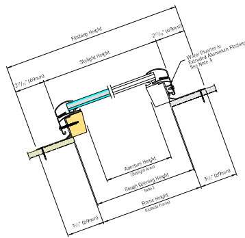
VERTICAL CROSS SECTION
